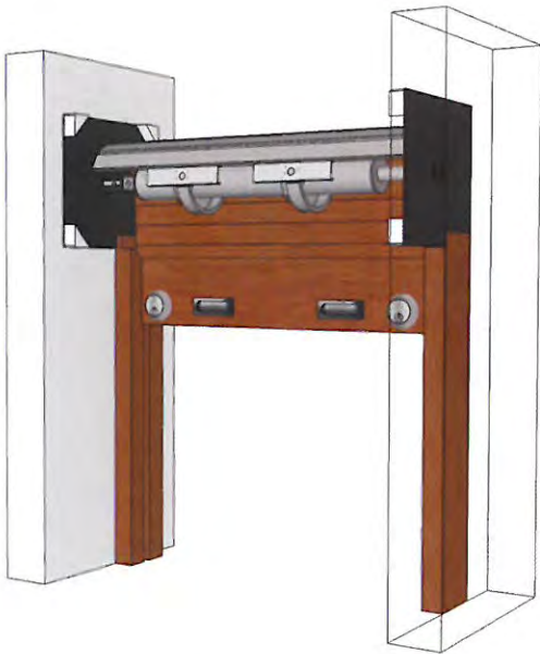
Between Wall Mount Without Lintel
