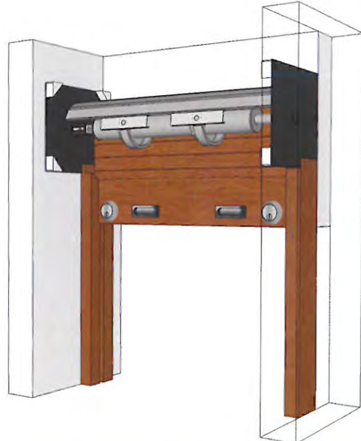
Between Wall Mount on Face of Lintel
